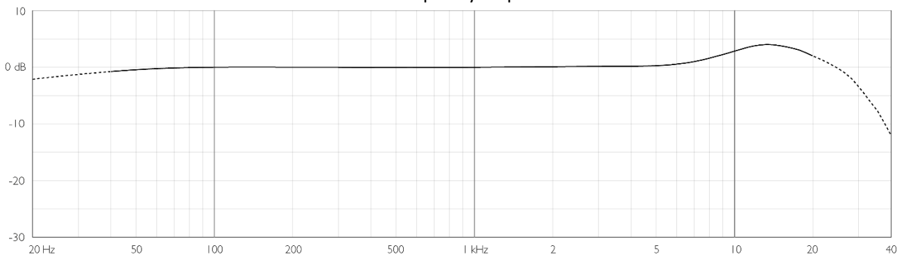
6060 Frequency response
